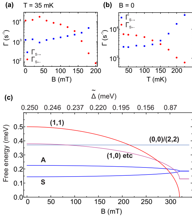
FIG. 4. (Color online) \Gamma_{S\rightarrow} and \Gamma_{S\leftarrow} as a function of (a) magnetic field at T = 35 mK, and (b) temperature at B = 0 . (c) Energy levels of device charge states at \delta = \epsilon = 0 as a function of B , showing the change in state ordering. Equivalent values of \tilde{\Delta} are shown on the top axis.
